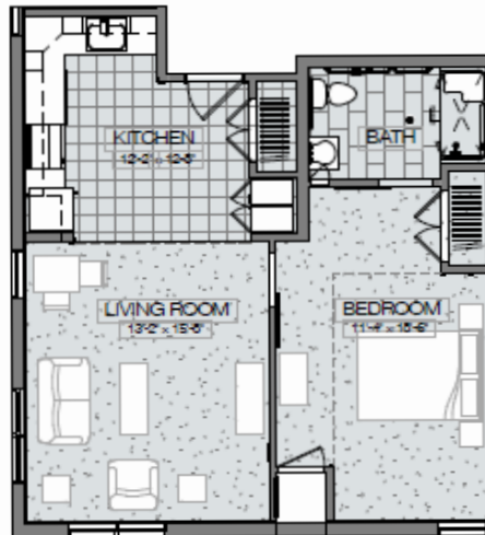
1 Typical One Bedroom Unit - Type A (HANDICAPPED ACCESSIBLE)
